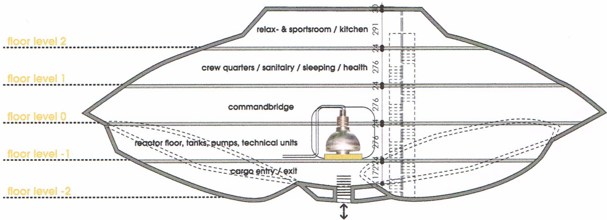
section: scale 1/200
